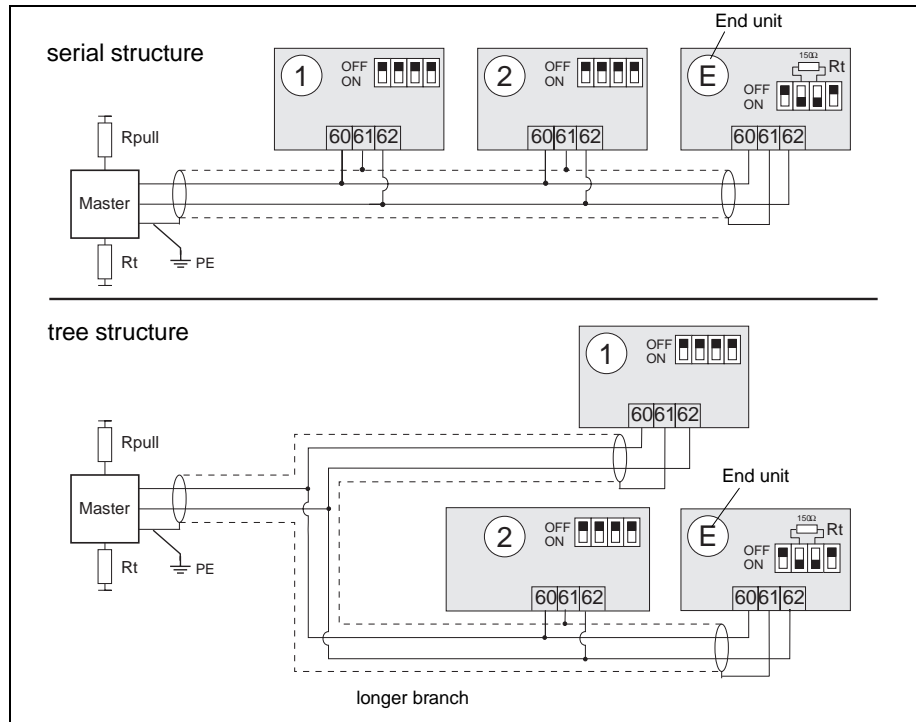
Bus topology. The master is a PC interface card or converter
