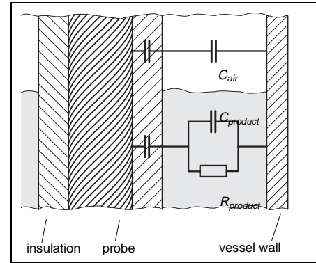
Capacitive measurement principle
