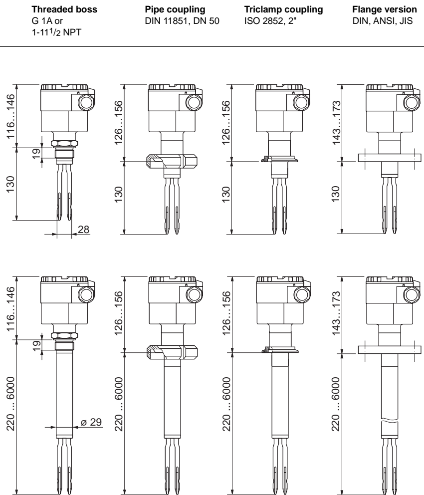
FTL 361 Extension tube version
